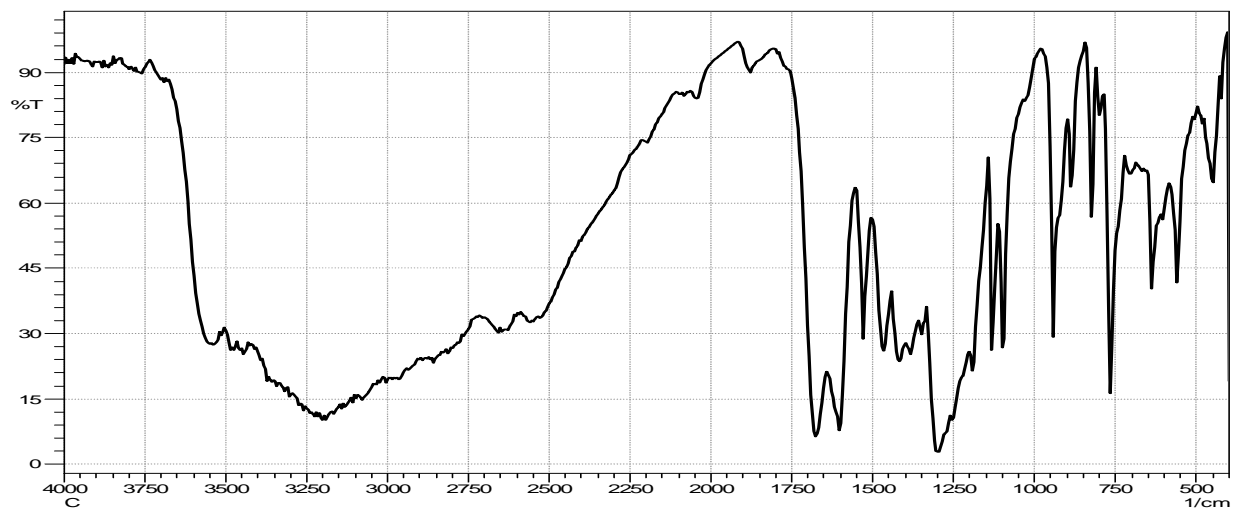
Fig. 2: IR spectrum of 2, 3-DHB
