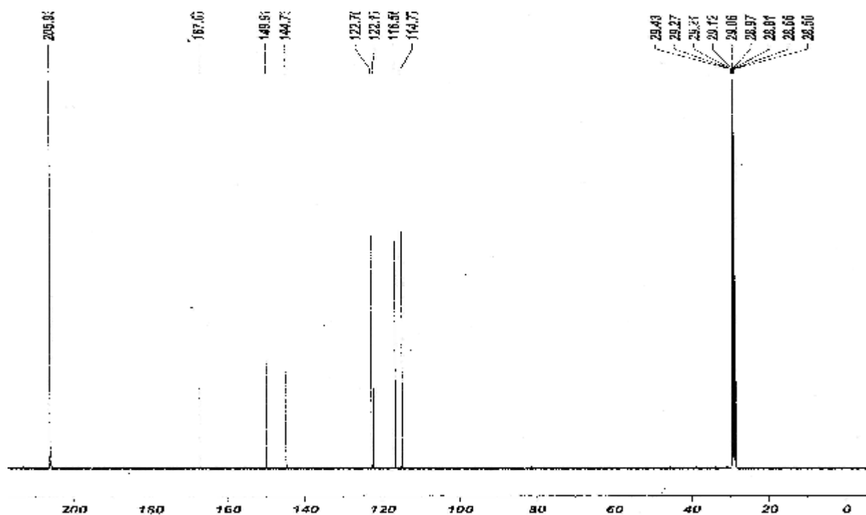
Fig. 4: ^{13}\text{C} NMR of 2, 3-DHB
