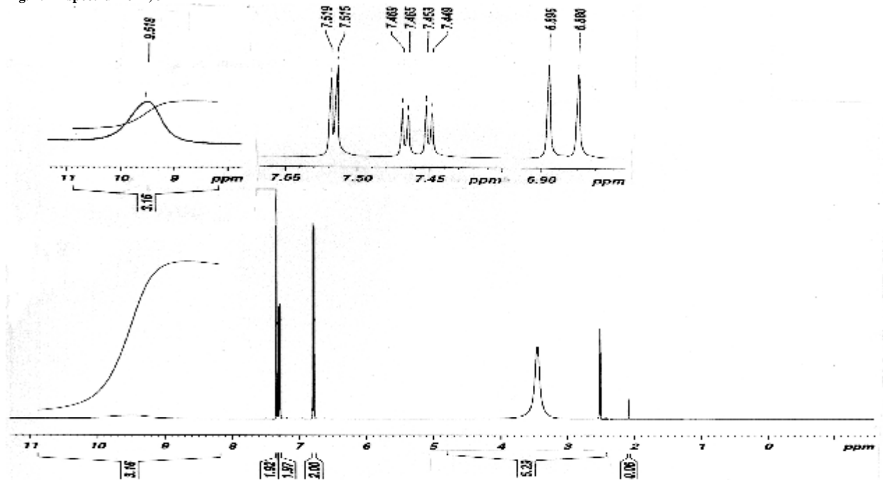
Fig. 3: 1 H NMR of 2, 3-DHB
