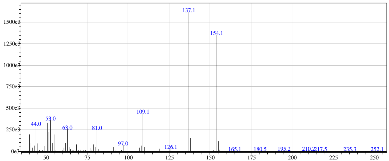
Fig. 1: Mass spectrum of 2, 3-DHB
